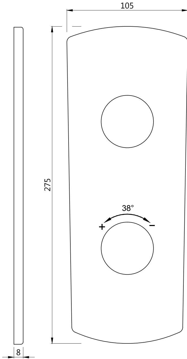
WALL FLANGE
