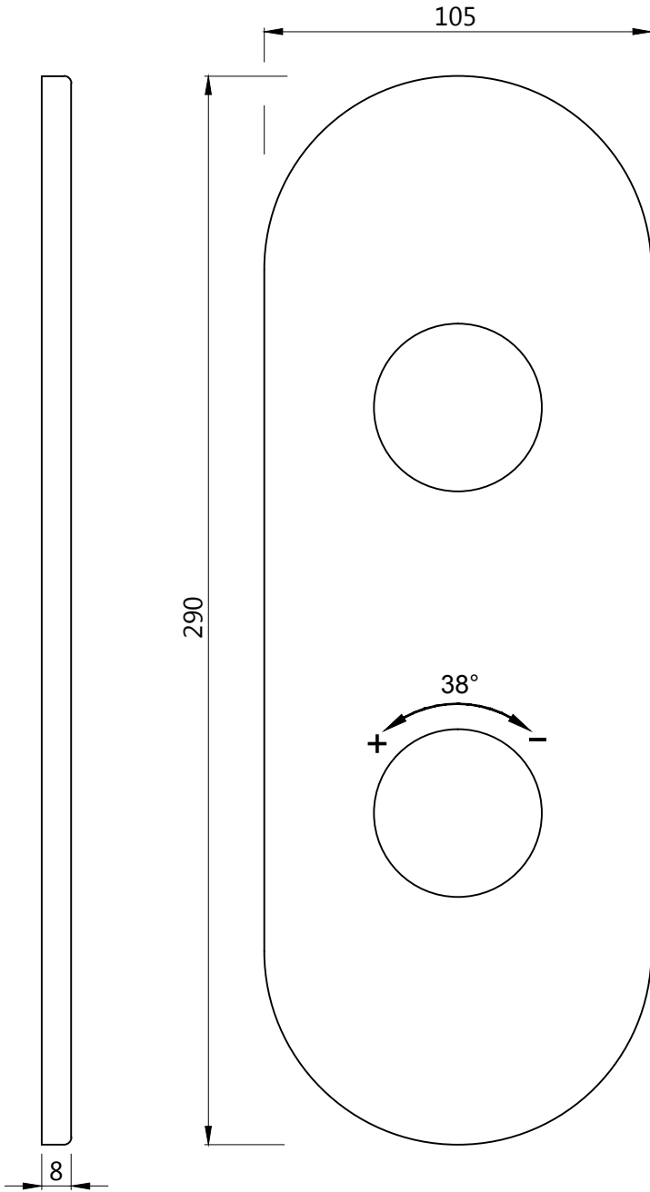
WALL FLANGE
