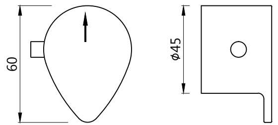
THERMOSTATE HANDLE
