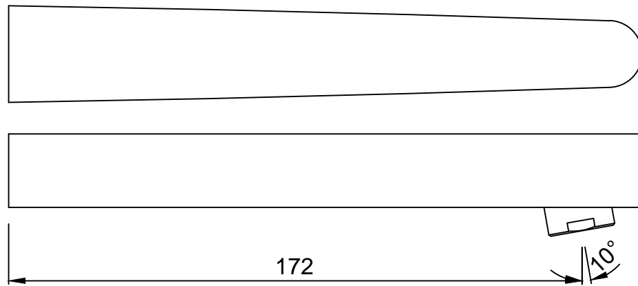
SPOUT
